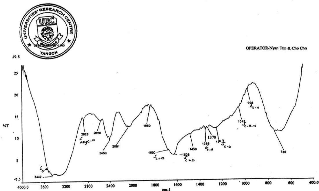
Figure 5. FT-IR spectral data of isolated compound 'B'
