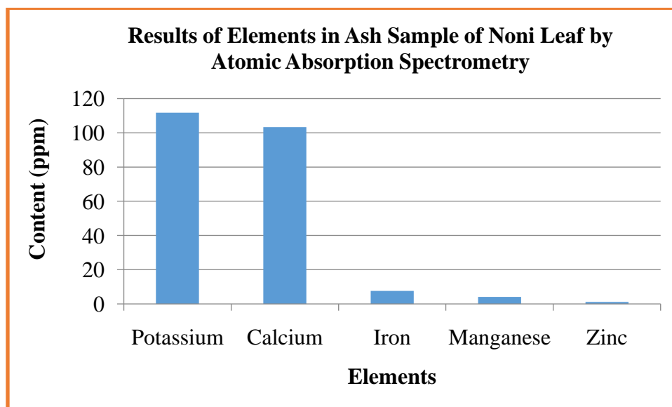
Figure 2. Quantitative result of some Element in Morinda angustifolia (Noni)
