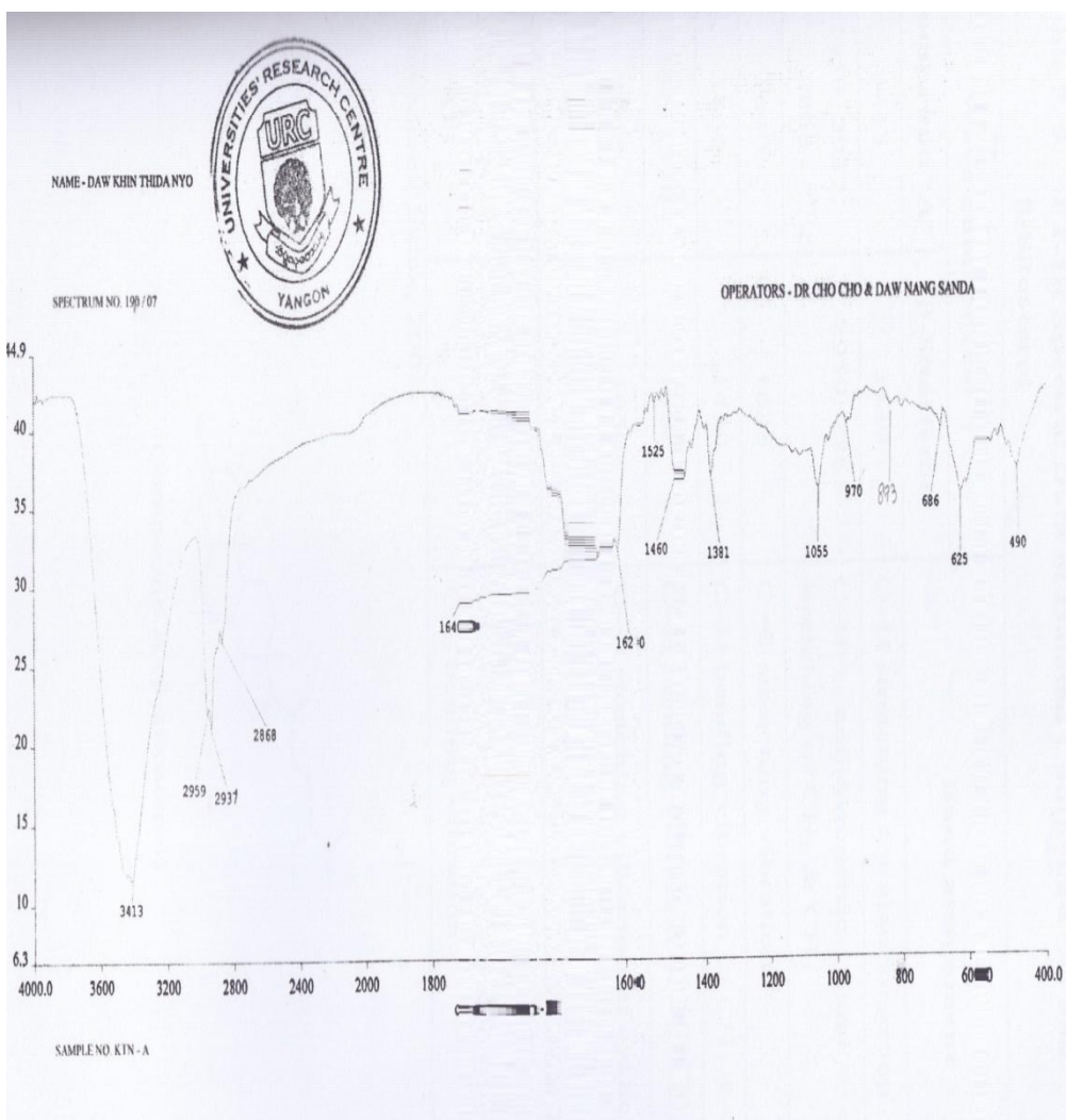
Figure 4. FT-IR spectral data of isolated compound 'A'
