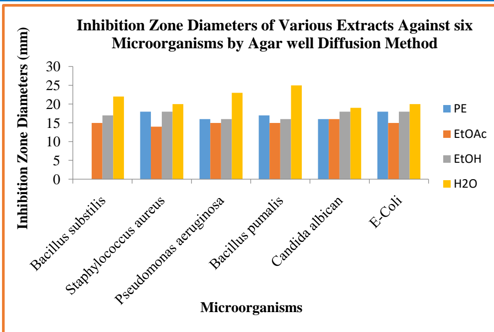
Figure 3. Evaluation on Antimicrobial Activities of Morindaangustifolia (Noni)
