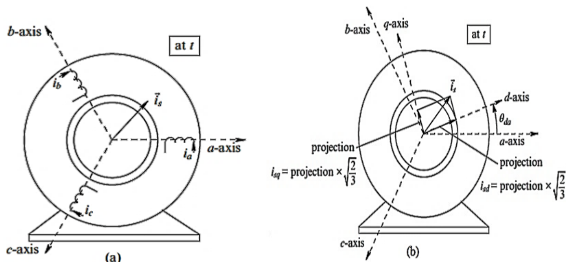
Figure 3. Representation of stator mmf by equivalent dq windings (Mohan, 2014)
