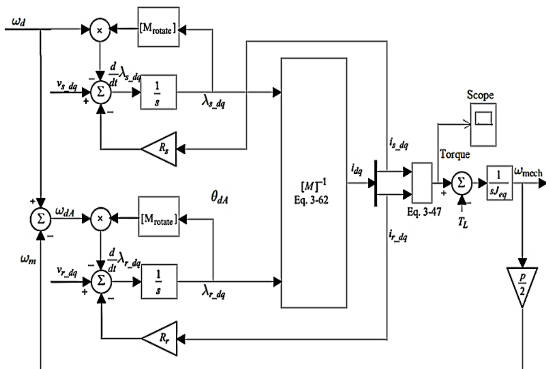
Figure 4. Induction motor model in terms of dq windings (Mohan, 2014)
