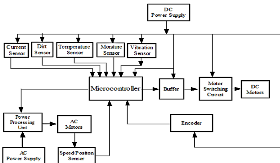
Figure 2. Block diagram of protection scheme against electric motors failure and for improved performance
