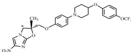
Figure 02: Molecular Structure of Delamanid
