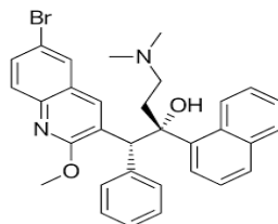
Figure 01: Molecular Structure of Bedaquiline
