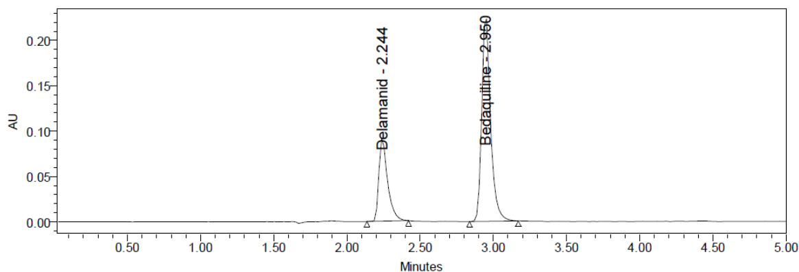
Figure 06: System suitability Chromatogram
