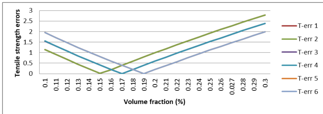
Figure 2. Ultimate tensile strength deviation errors
