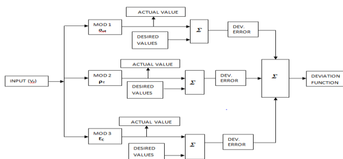
Figure 1. Simulink System Block
