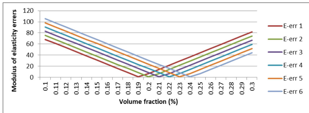
Figure 3. Modulus of elasticity deviation errors
